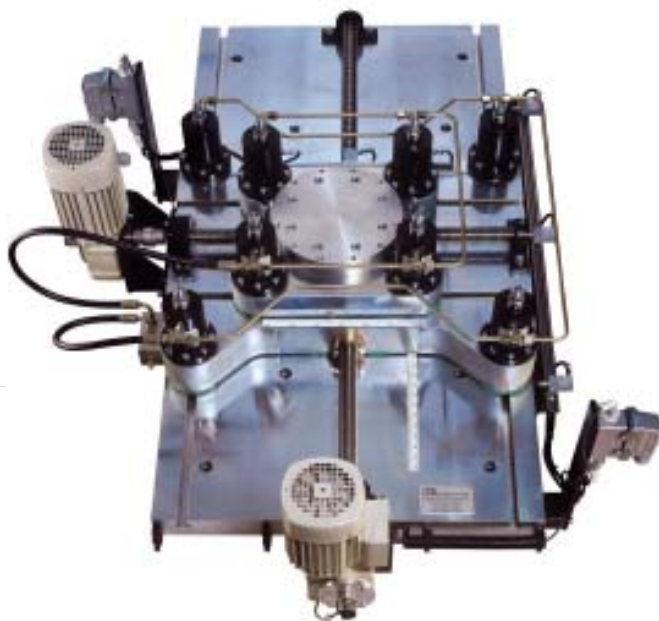
X-Y-positioner unit
