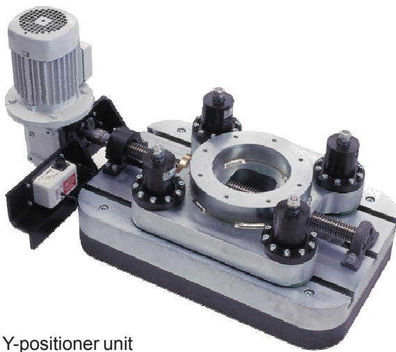
X-Y-positioner unit
